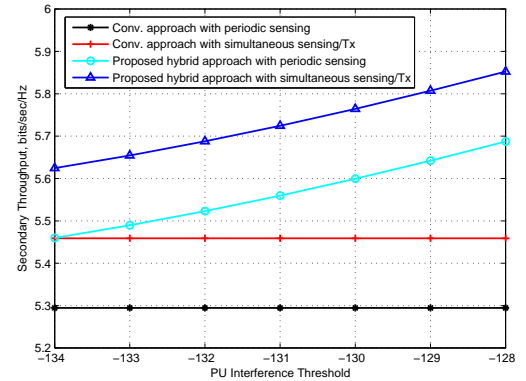
Fig. 6: Secondary throughput versus PU interference threshold for different approaches ( \bar{\mathcal{P}}_d = 0.9 , T = 100 ms, \text{SNR}_p = -15 dB, \text{SNR}_s = 20 dB, \tau = 2.5 ms)
