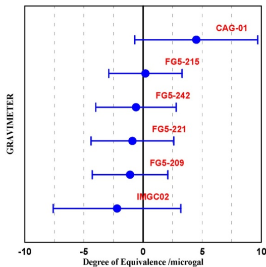
Figure 2: Degrees of Equivalence (DoE) of the gravimeters participating in the KC using the gravity differences between the sites from all gravimeters. Absolute measurements corrected for the self-attraction, laser beam diffraction effects and geophysical gravity changes observed with the SG.
