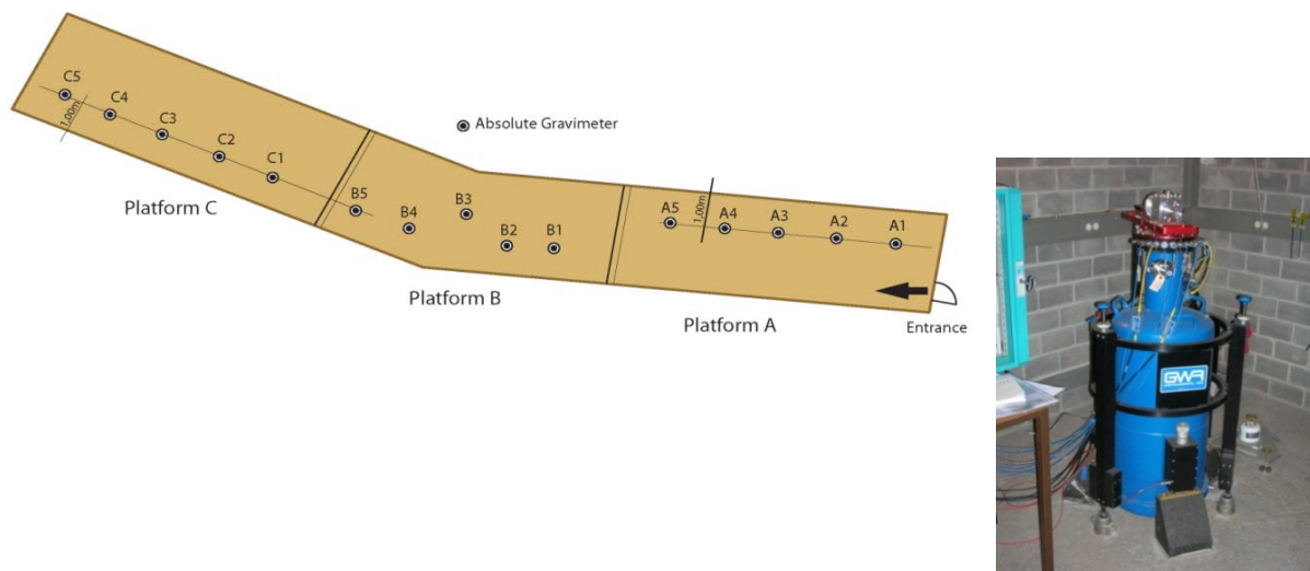
Figure 1: Sketch of the underground laboratory allowing for the simultaneous set up of 15 gravimeters (40 m length and 3.6 m wide) and the superconducting gravimeter OSG-CT040.
