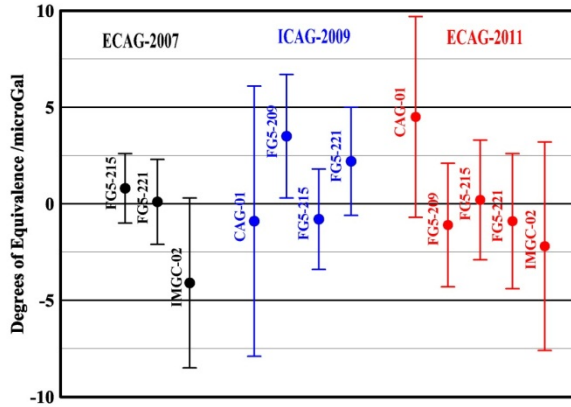
Figure 3: Degrees of Equivalence for the KC gravimeters which participated in ECAG-2007, ICAG-2009 and ECAG-2011.
