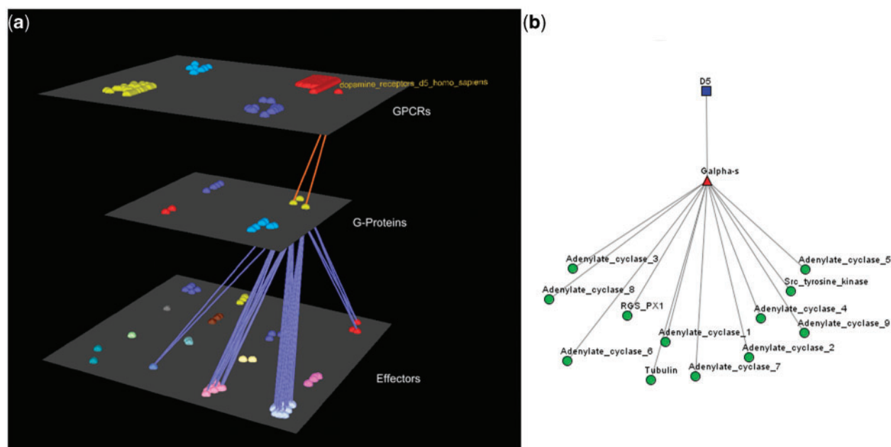
Figure 3. Visualization of human Dopamine D5 receptor's interactions. (a) Arena3D Visualization: Human Dopamine D5 receptor targets two G\alpha-s G-Proteins. The G-Proteins are connected to 12 types of effectors belonging to four specific families. These are: Adenylate cyclases, Regulators of G-Protein signaling, Tyr protein kinases and tubulins. (b) Medusa 2D Visualization: human dopamine D5 receptor targets G\alpha-s G-Proteins, which interact with the following four families of effectors: Adenylate cyclases, Regulators of G-Protein signaling, Tyr protein kinases and tubulins.
