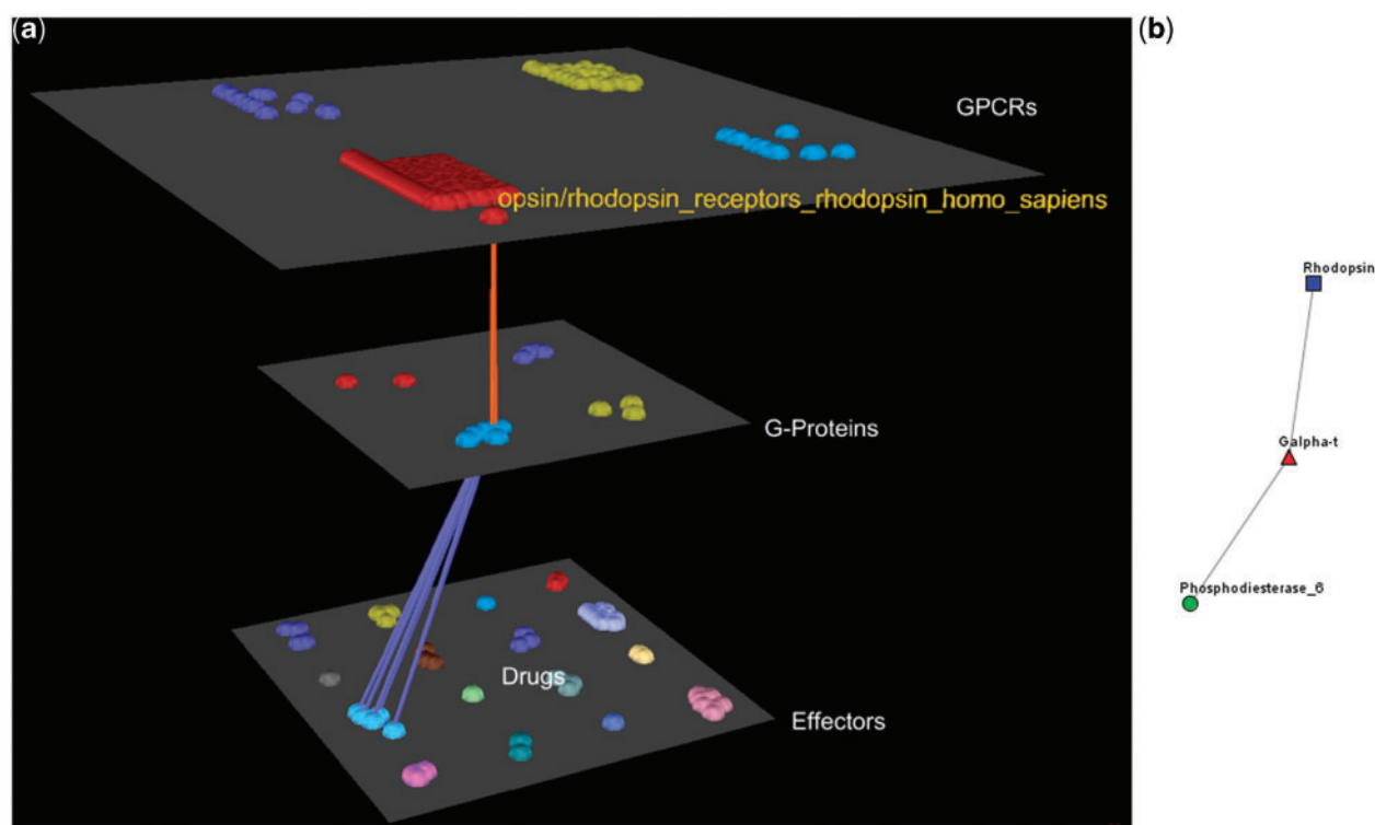
Figure 4. Visualization of human Rhodopsin receptors' interactions. (a) Arena3D Visualization: Human Rhodopsin receptor targets three G\alpha G-Proteins that belong to the G\alpha -t subfamily. The three G-Proteins interact with five effectors belonging to the Rhodopsin-sensitive cGMP-specific PDEases subfamily and more specifically to Phosphodiesterase 6 type of effectors. (b) Medusa 2D Visualization: the Rhodopsin subfamily of the Opsin/Rhodopsin family of the Class A of the GPCRs interacts with the G\alpha -t subfamily of the G-Proteins which interact with the Rhodopsin-sensitive cGMP-specific PDEases effectors' subfamily.
