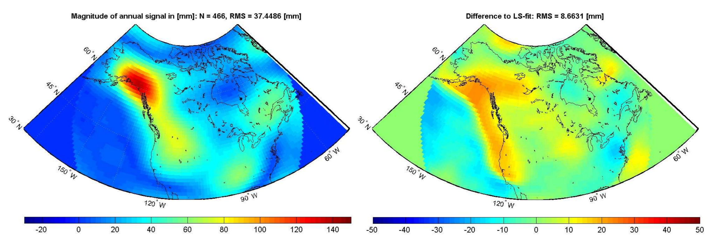
Figure 4: Magnitude of the annual cycle in equivalent water height
