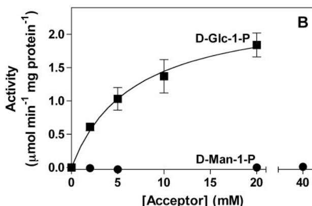
FIGURE 5. Effect of P_i , D-Glc-1-P, and D-Man-1-P concentrations on the activity of recombinant VTC5. GDP-L-Gal phosphorylase and GDP-L-Gal-hexose-1-phosphate guanylyltransferase activities of VTC5 were assayed under the same conditions as those of VTC2 (see Fig. 4). The curves shown represent ideal saturation curves obtained by fitting the activities measured in the presence of P_i and D-Glc-1-P to the Michaelis-Menten equation. The axis scales in panels A and B have been drawn to highlight the high and low activities found. Activities are the means \pm S.D. values calculated from two (activity with D-Man-1-P) or three (activities with P_i or D-Glc-1-P) separate experiments.
