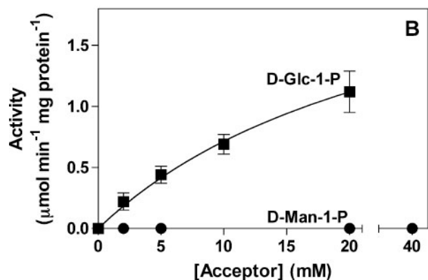
FIGURE 4. Effect of P_i , D-Glc-1-P, and D-Man-1-P concentrations on the activity of recombinant VTC2. GDP-L-Gal phosphorylase and GDP-L-Gal-hexose-1-phosphate guanylyltransferase activities were assayed as described under "Experimental Procedures" in the presence of 25 \mu\text{M} GDP-L-Gal and the indicated concentrations of P_i , D-Glc-1-P, or D-Man-1-P. Reactions were stopped 10 min after the addition of recombinant VTC2. The curves shown represent ideal saturation curves obtained by fitting the activities measured in the presence of P_i and D-Glc-1-P to the Michaelis-Menten equation. The axis scales in panels A and B have been drawn to highlight the high and low activities found. Activities are the means \pm S.D. values calculated from at least three separate experiments.
