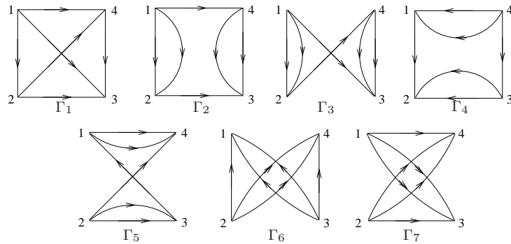
Figure 4: Wick's contraction
