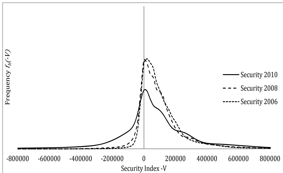
Panel B: Italy \gamma = 5
