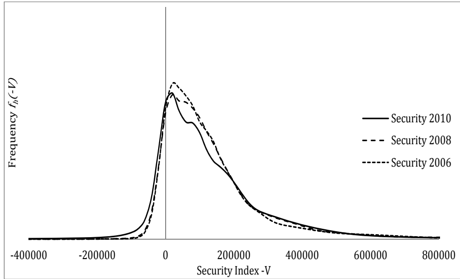
Panel A: Italy \gamma = 1
