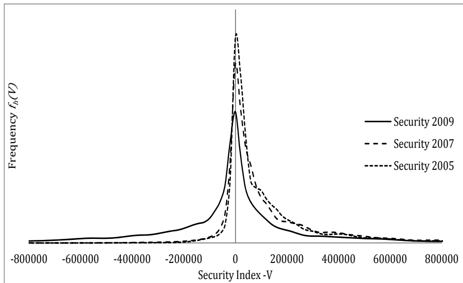
Panel B: USA \gamma = 5
