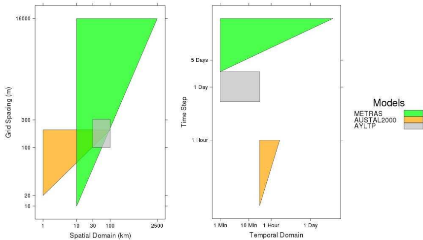
Figure 3: Space (left figure) and time (right figure) comparison of METRAS and AUSTAL2000 models with AYLTP.
