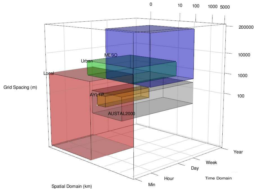
Figure 1: Schematic representation of air pollution model's scales. The red cube represents the local scale models, the green represents the urban scale, the blue the mesoscale, the orange stands for the AYLTP requirements and the grey describes AUSTAL2000.
