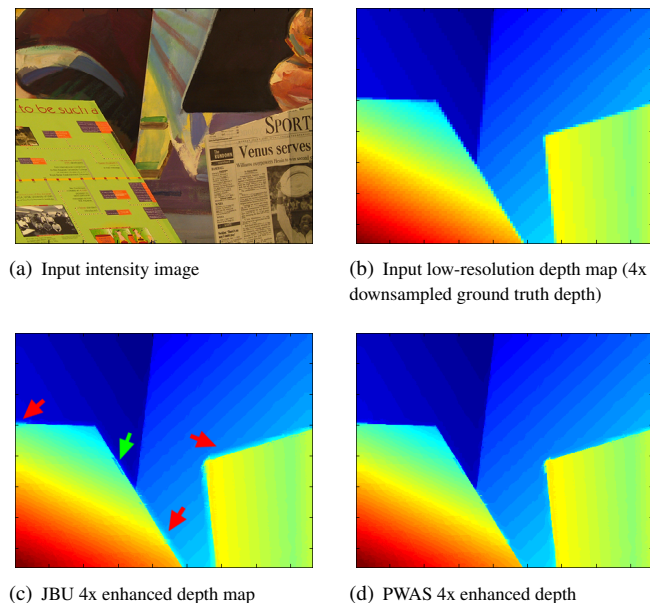
Fig. 4. Although JBU and our method increase the low-resolution depth map to the input guidance image, in contrast to our result, the JBU performance exhibits slight texture copy and edge blurring in the areas marked with green and red arrows, respectively.
