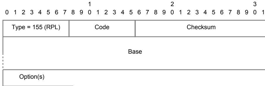
Fig. 5. RPL encapsulation in an ICMPv6 packet.
