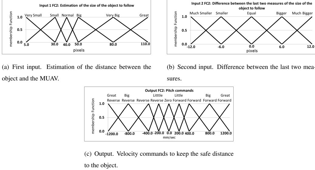
Figure 4: Definition of the Pitch controller.
