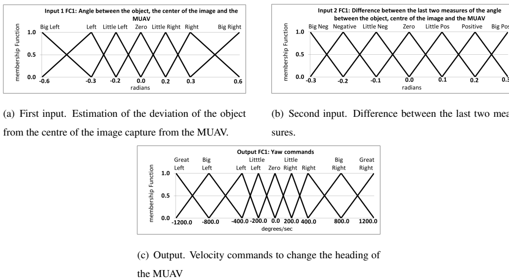
Figure 3: Definition of the Yaw controller.
