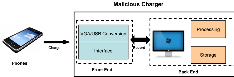
Fig. 1. The high-level architecture of juice filing charging attack.
