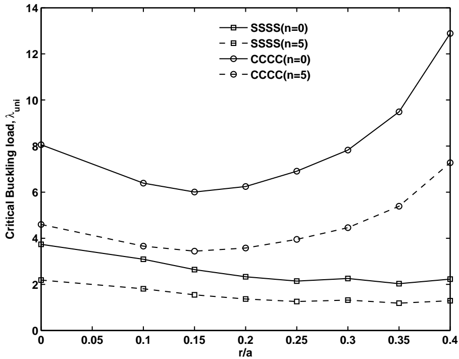
Figure 8: Variation of the critical buckling load, \lambda_{cr} = \frac{N_{xx}^0 b^2}{\pi^2 D_c} with cutout dimensions for a square FGM plate with a/h=10 subjected to uniaxial compressive loading for different gradient index n and various boundary conditions.
